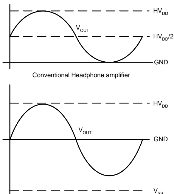
Cap-free Headphone amplifier Figure 2: Cap-free Operation
